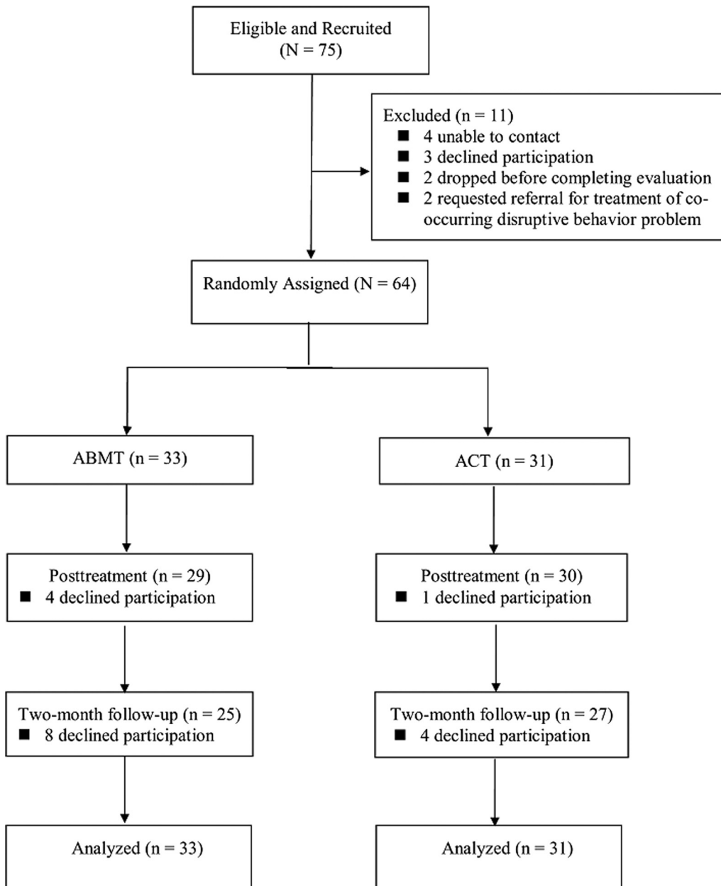
FIGURE 1 CONSORT Diagram
