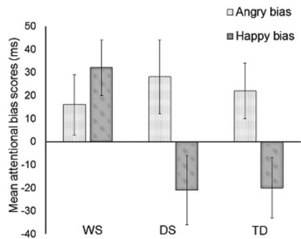
Figure 2. Mean attentional bias scores with standard error (ms).
