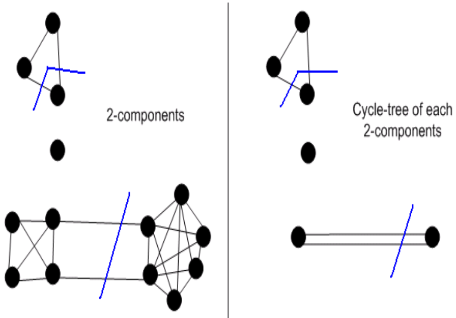
Figure 5. The 2-classes and their corresponding cycle-tree connectivity models (the induced graph presented in Fig. 4)
