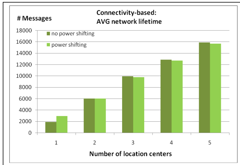
Figure 13. The average network lifetime of the connectivity-based algorithm with and without the connectivity-based initial power assignment, according to the number of location centers in the network topology.
