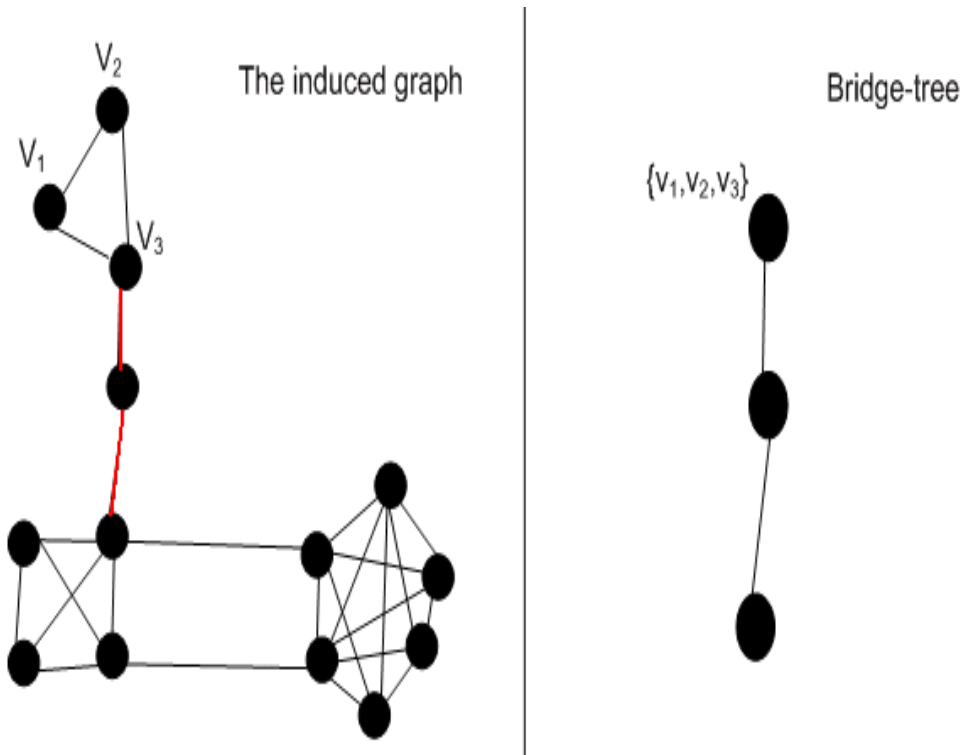
Figure 3. An example of a 2-class and its subdivision into 3-classes.
