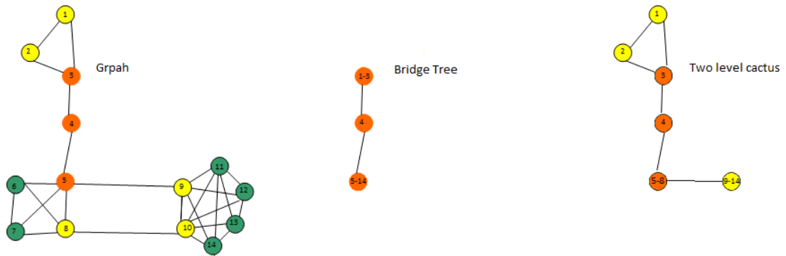
Figure 8. The priority nodes identified by the different models
