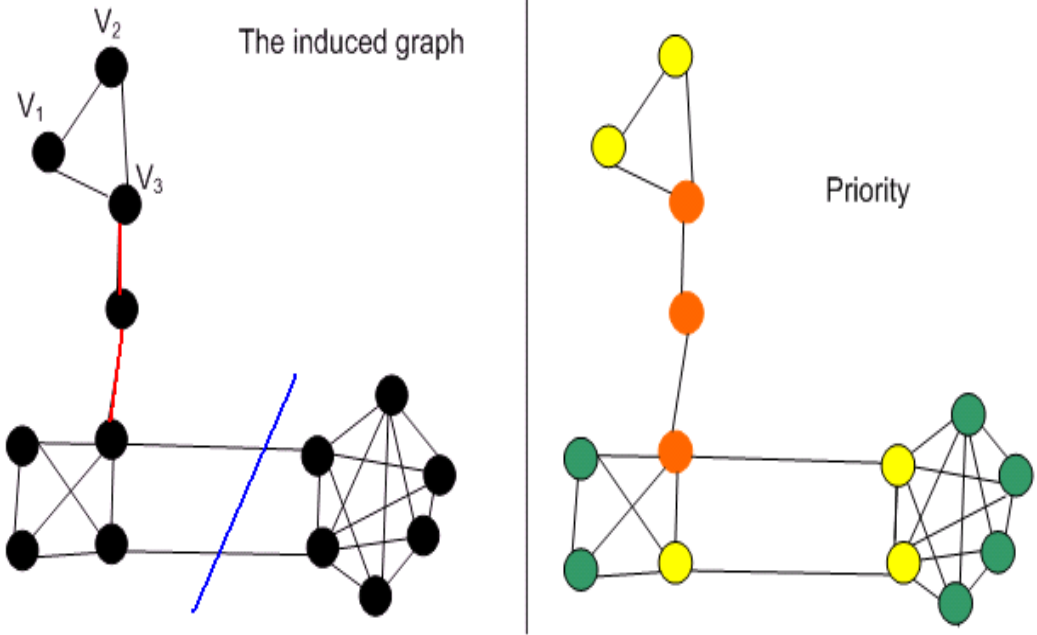
Figure 7. The priority assignment
