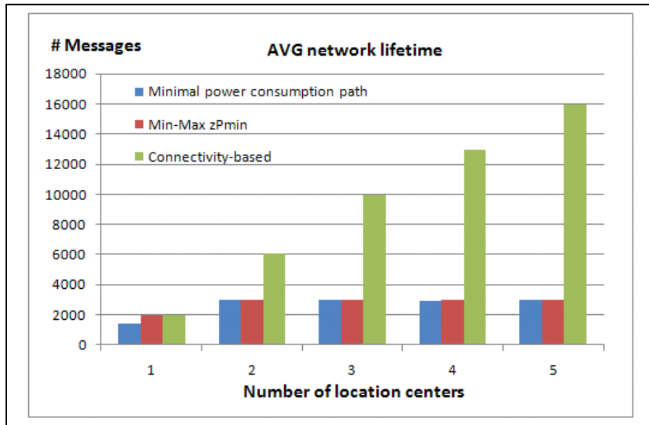
Figure 10. The average network lifetime according to the number of location centers in the network topology.
