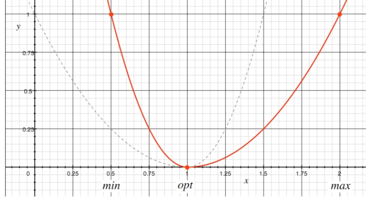
Figure 6.1: Normalization function - the red curve shows the normalization function and the grey dotted line shows the rest of the half-functions used to produce the normalizing functions. The three operating limits are highlighted by red dots, where in this example m = 0.5 , \sigma = 1 , and m = 2 .
