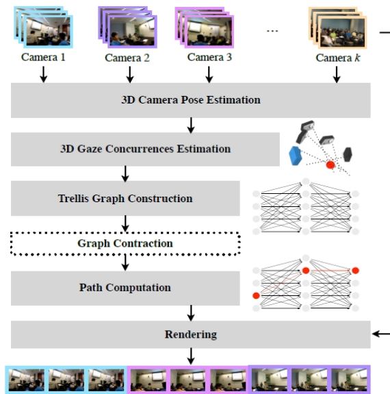
Figure 3.1: Our method’s pipeline: from multiple camera feeds to a single output “cut”.
