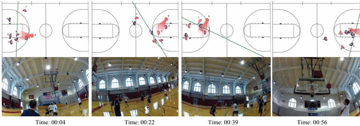
Figure 4.3: 3D reconstruction of the camera position and orientation allows our algorithm to track the joint attention through the basketball game. The blue dot in the top view of the reconstructions is the joint attention point. One can see how most players are watching the same position in the scene (usually the ball position), which is the focus of joint attention during the game. The green line is the 180-line according to the current camera (see also Figure 1.1).
