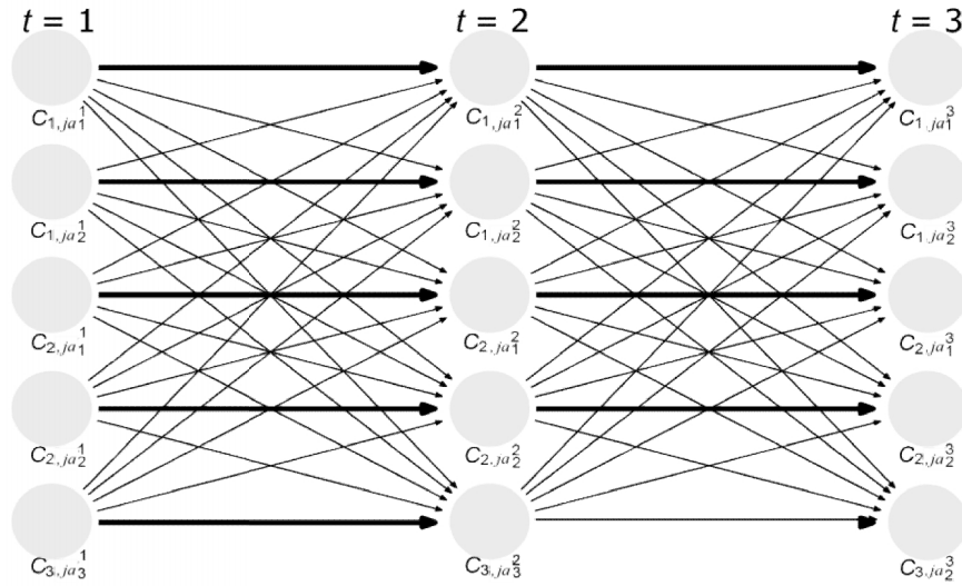
Figure 6.2: The trellis structure used in our algorithm; the frames are nodes (C_j, ja_i^t) for time t , camera C_j and 3D joint attention ja_i^t with two types of edges: continuous (bold) and transition edges. In this example, at each time t there are three synchronized camera sources C_1 , C_2 , and C_3 and there are three joint attention points ja_1 , ja_2 , and ja_3 . Assume that ja_1^t and ja_2^t project onto C_1 and C_2 and ja_3^t on C_3 , for t = 1 and 2 . Further, assume that the third point of 3D joint attention ja_3^3 ceases to exist as a point of interest at t = 3 , and camera C_3 views ja_2^3 instead. The graph contains a set of five nodes for every slice S_t as follows: S_t = \{(C_1, ja_1^t), (C_1, ja_2^t), (C_2, ja_1^t), (C_2, ja_2^t), (C_3, ja_3^t)\} for the first two time instances, and S_3 = \{(C_1, ja_1^3), (C_1, ja_2^3), (C_2, ja_1^3), (C_2, ja_2^3), (C_3, ja_2^3)\} for t = 3 .
