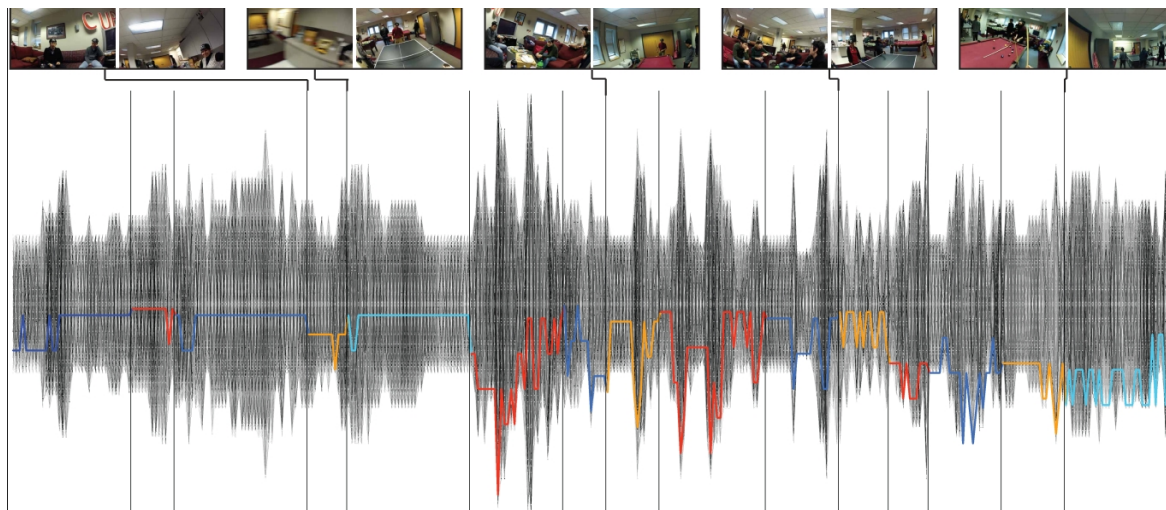
Figure 9.8: The four-scene party footage graph expands and contracts because of the dynamic nature of the party scene – people are moving around and the point of 3D joint attention changes. Our algorithm can detect four sub-scenes by clustering the points of 3D joint attention spatially (each color in the path denotes a sub-scene), and creates a coherent story merging the four without jumping too much from one to another. At the top we illustrate some cuts from one sub-scene to another.
