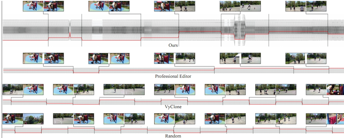
Figure 9.2: Visualization of the movie cut created by different methods for the Park sequence where two distinct sub-scenes are taking place very close to each other in the same area: a basketball game and a kid playing in a playground. Our trellis graph is portrayed below the images and the path chosen is shown in red. The graph includes a node for each point of 3D joint attention and each zoom level and expands when more points of joint attention are found. For the other methods, the graph only includes nodes for each camera. Note that the edited videos produced by VyClone and the Random method look similar in that the time between cuts is almost constant rather than changing to reflect the pace of the action. Neither approach handles this scene well because the edited videos cut three or four times from one sub-scene to the other, creating a confusing version of the event. In our edited video and the hand-edited one, the cuts are much more varied in length and there is one transition from the playground to the basketball game.
